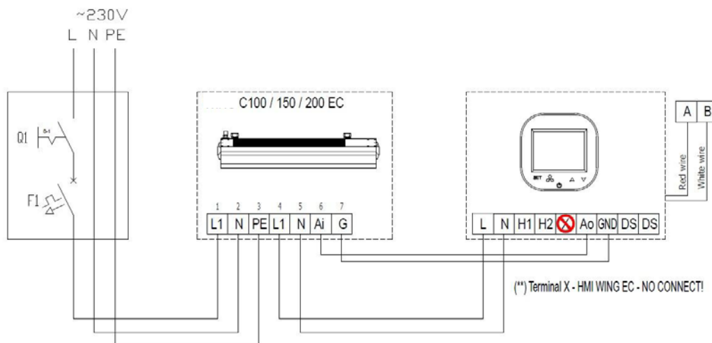
Figura 5 – Conexiuni EASYAIR C100/150/200
