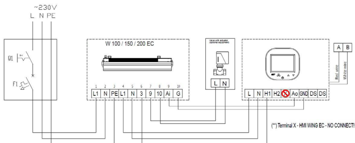
Figure 1 - Raccordement EASYAIR W100/150/200
