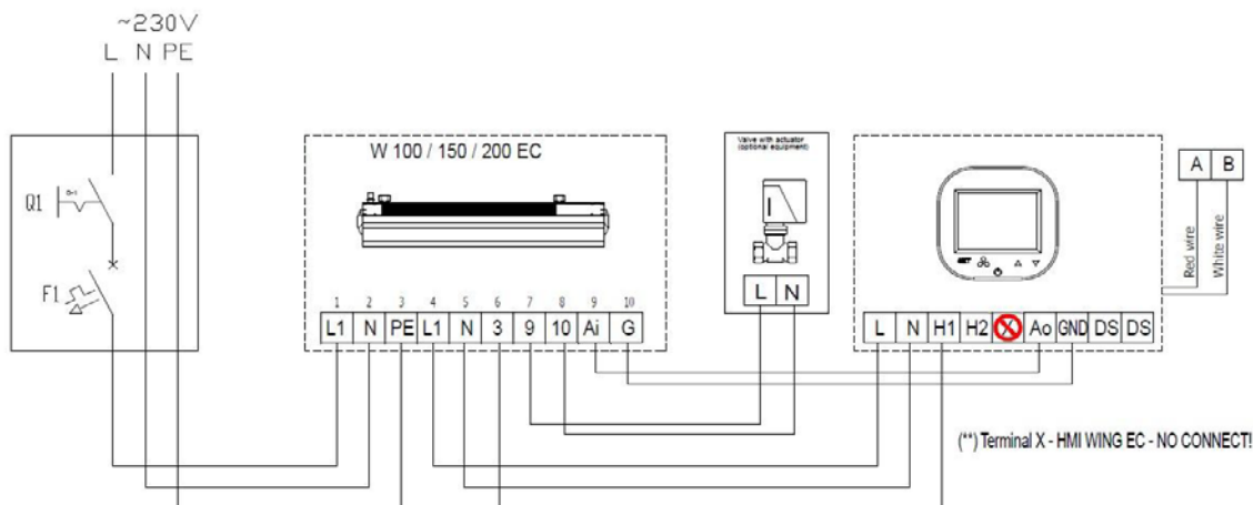
Figura 1 – Conexiuni EASYAIR W100/150/200
