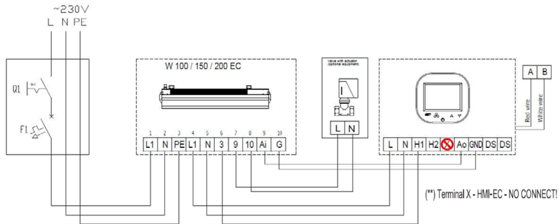
Figure 2 - EASYAIR W100/150/200 connections
