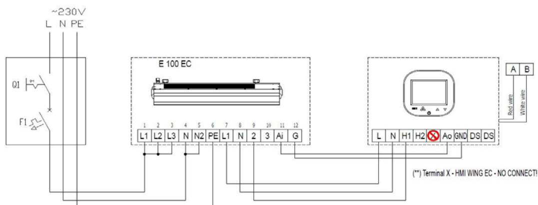
Figure 3 - Raccordement EASYAIR E100
