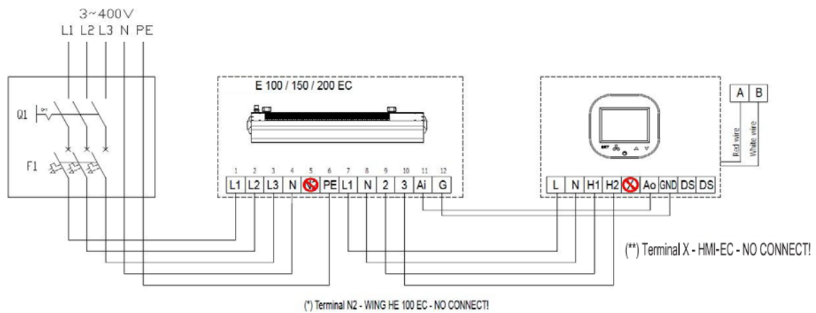
Figure 3 - EASYAIR E100/150/200 connections
