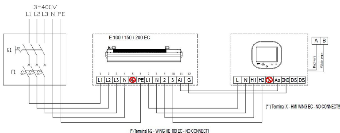
Figure 2 - Raccordement EASYAIR E100/150/200
