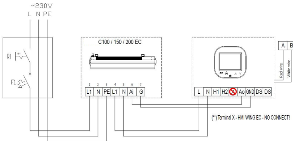
Figure 5 - EASYAIR C100/150/200
