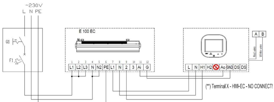
Figure 4 - EASYAIR E100 connections
