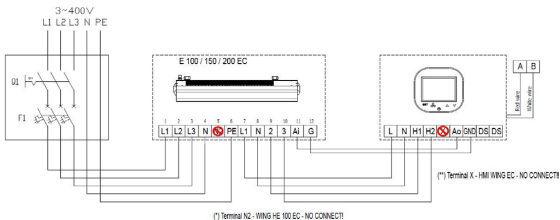
Figura 2 - Conexiuni EASYAIR E100/150/200
